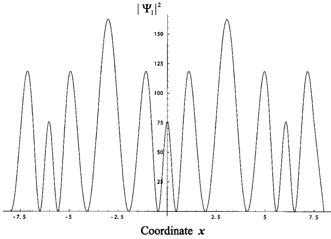
FIG. 1. Square of the modulus of the amplitude |\psi_1|^2 versus the coordinate x , Eq. (14), k=0.98 , \delta_1=-4.63 , c_1=-2.06 , r=1 .
